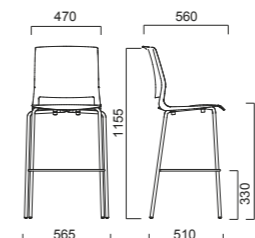
SOL 4-LEG STOOL
