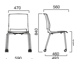
SOL 4 LEGS WITH CASTORS
