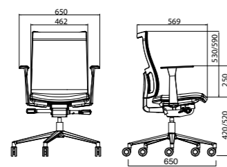
STEP WITH MESH BACKREST WITH FIXED ARMS
