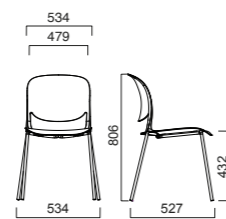
OUTLINE 4 LEGS
