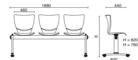
MONO 170 ON 500 BENCH
