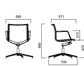
ALUMINIA LOW BACK WITH ARMRESTS FOR MESH UPHOLSTERY
