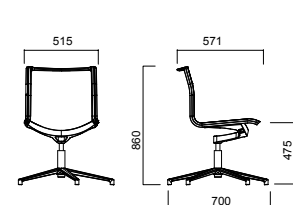
ALUMINIA LOW BACK WITHOUT ARMRESTS FOR UPHOLSTERY
