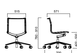
ALUMINIA LOW BACK WITHOUT ARMRESTS FOR MESH UPHOLSTERY
