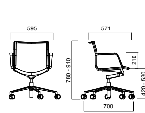
ALUMINIA LOW BACK WITH ARMRESTS FOR UPHOLSTERY
