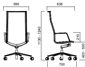
ALUMINIA HIGH BACK FOR UPHOLSTERY AND TILTING MECHANISM
