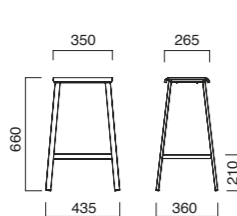
KD KITCHEN STOOL
