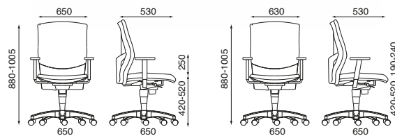
ONLINE WITH ARMRESTS FOR UPHOLSTERY
